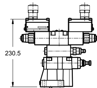
RQM3K*-P*/D/10*-K9T*
